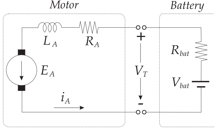
Figure 5.11: DC Motor and Battery Model
