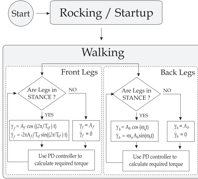
Figure 4.12: Walking controller flow chart
