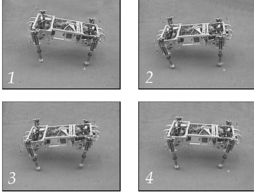
Figure 5.6: Key frames of Scout II in a bounding walk. Four distinct phases are observable : 1) Single Support (Back), 2) Double Support (Back to Front), 3) Single Support (Front), and 4) Double Support (Front to Back)
