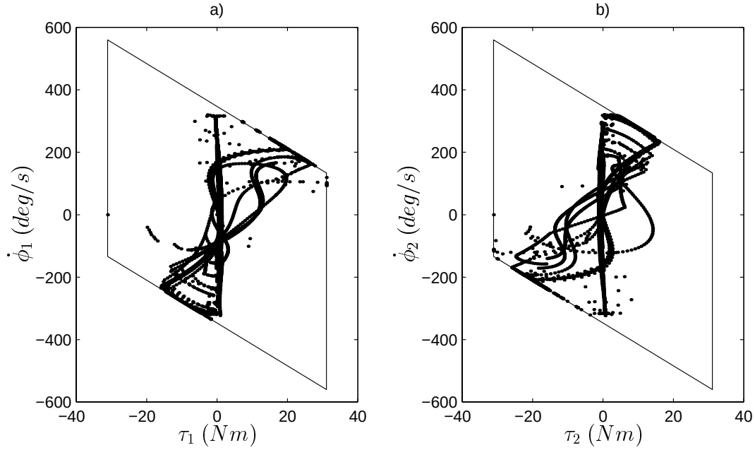
Figure 4.9: Simulation torque/speed motor model. Actual Torque vs. \dot{\phi} for the a) Front and b) Back legs.
